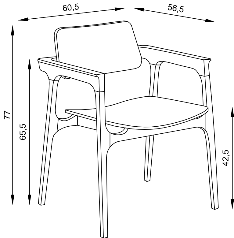
CADEIRA DITTA MADEIRA
